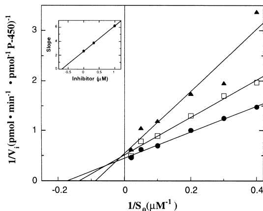
Figure 3. Inhibition of 18-hydroxylase activity of bovine P -450 11 \beta by 18-VDOC. 18-Hydroxylase activity of bovine P -450 11 \beta (450 nM) was studied with [ ^3 H]corticosterone as substrate (2.5–50 \mu M), without (●) or with 18-VDOC at 0.33 \mu M (□), or 1 \mu M (▲). Shown is a representative graph of at least two independent determinations. Duplicate measurements were run for each experiment.
