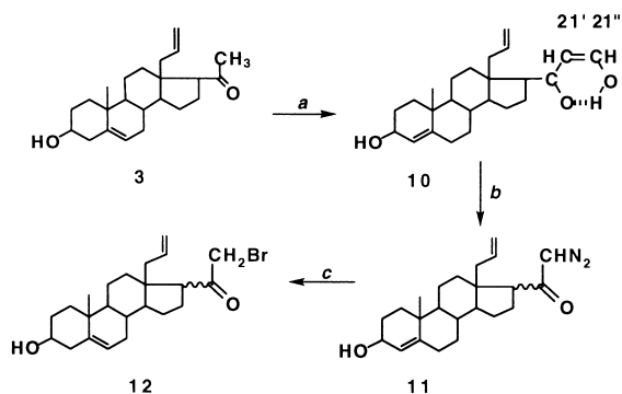
Scheme 4. (a) NaH, \text{C}_2\text{H}_5 , \text{HCOOEt} , THF; (b) \text{TsN}_3 , NaH, \text{C}_2\text{H}_5\text{OH} , THF; (c) KBr, TsOH, \text{H}_2\text{O} , \text{CH}_3\text{CN} .
