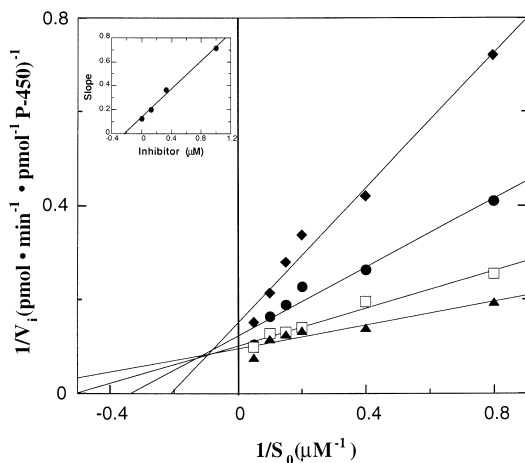
Figure 2. Inhibition of 11 \beta -hydroxylase activity of bovine P -450 11 \beta by 18-VDOC. 11 \beta -Hydroxylase activity of bovine P -450 11 \beta (40 nM) was studied with [ ^{14} C]11-deoxycorticosterone as substrate (1.25–20 \mu M), without (▲) or with 18-VDOC at 0.125 \mu M (□), 0.33 \mu M (●), or 1 \mu M (◆). Shown is a representative graph of at least two independent determinations. Duplicate measurements were run for each experiment.
