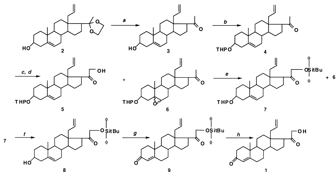
Scheme 3. (a) p TosOH, acetone; (b) dihydropyran, PPTS, \text{CH}_2\text{Cl}_2 ; (c) LDA, THF, \text{Me}_3\text{SiCl} ; (d) MMPP, ethanol; (e) t BuPh 2 SiCl, DMAP, pyridine, \text{CH}_2\text{Cl}_2 ; (f) AcOH, \text{H}_2\text{O} , THF; (g) N -Me piperidone, THF, \text{Al}(\text{O}i\text{Pr})_3 ; (h) HCl, methanol.
