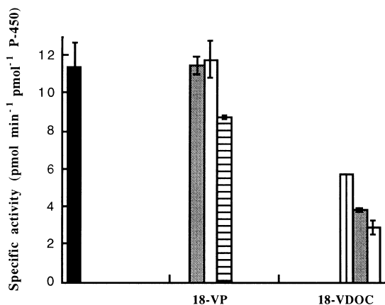
Figure 1. Inhibition of the transformation of DOC to corticosterone by 18-VP or 18-VDOC. 11 \beta -Hydroxylase activity of bovine P -450 11 \beta (20 nM) was measured in a reaction mixture containing [ ^{14} C]11-deoxycorticosterone as substrate (1.25 \mu M) in the presence of inhibitors 18-VP or 18-VDOC at concentrations of: 0.25 \mu M (□), 0.5 \mu M (▨), 1 \mu M (▤), or 10 \mu M (▧). 100% is the production without inhibitor (■). Each activity is the average of duplicate measurements in the same experiment. Shown is a representative example of two independent experiments.
